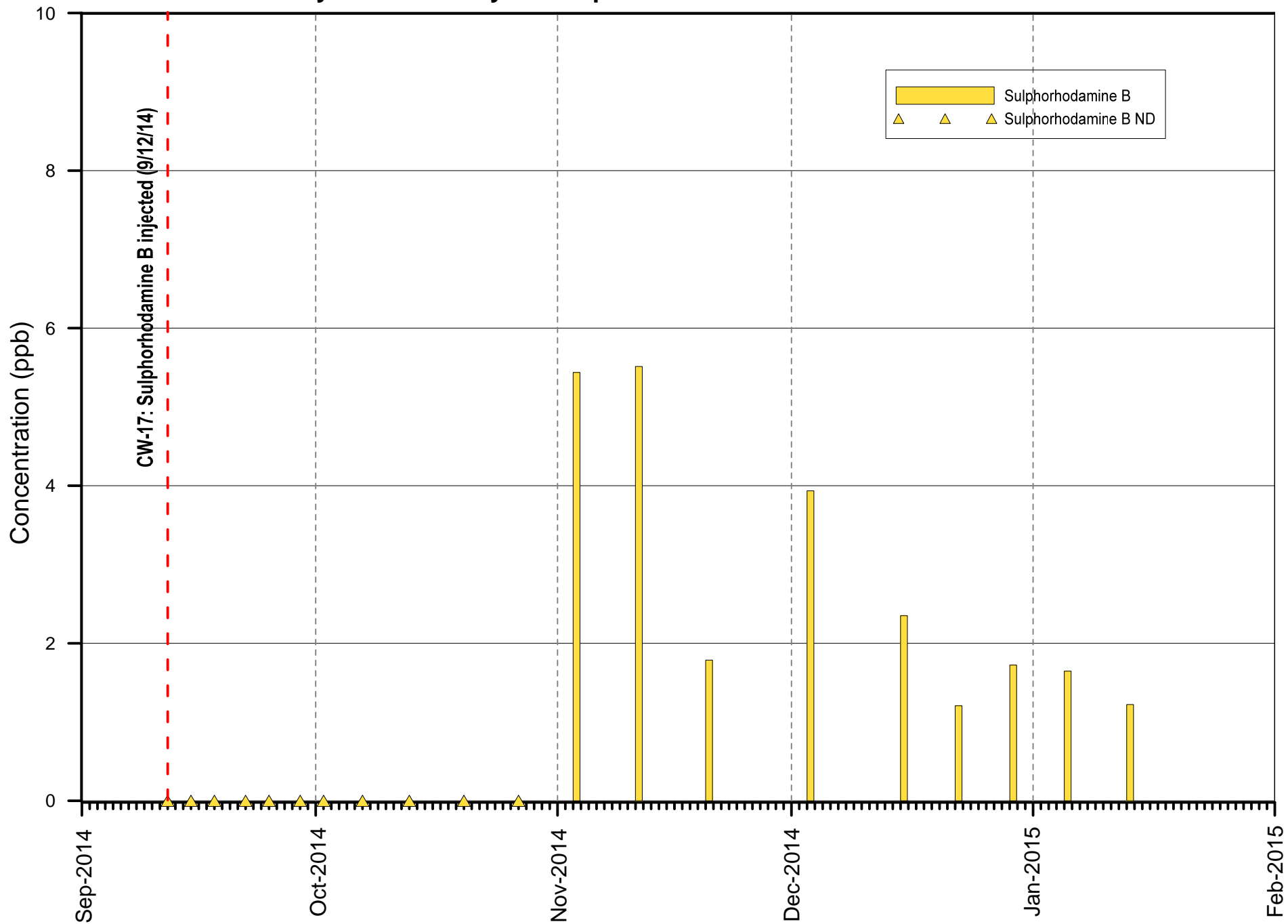
Figure 3.2-6 SW-13 Dye Tracer Analysis Sulphorhodamine B Detections - 2nd Test at CW-17
